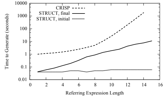
Figure 2: Experimental comparison between STRUCT and CRISP: Generation time vs. length of referring expression
