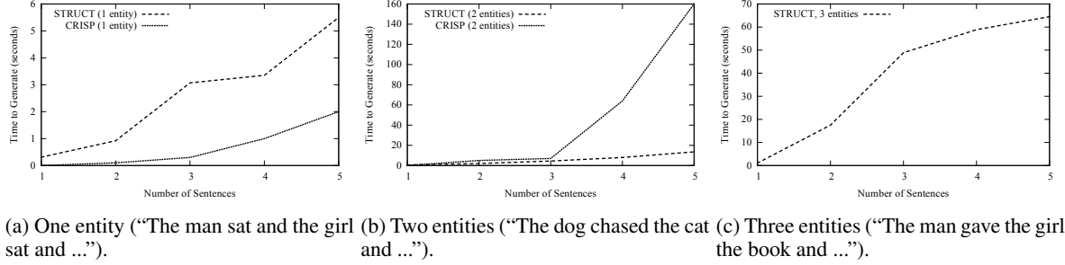
Figure 4: Time taken by STRUCT to generate sentences with conjunctions with varying numbers of entities.
