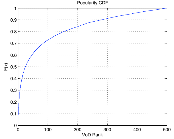
Fig. 6 VoD simulated popularity - Zipf distribution
