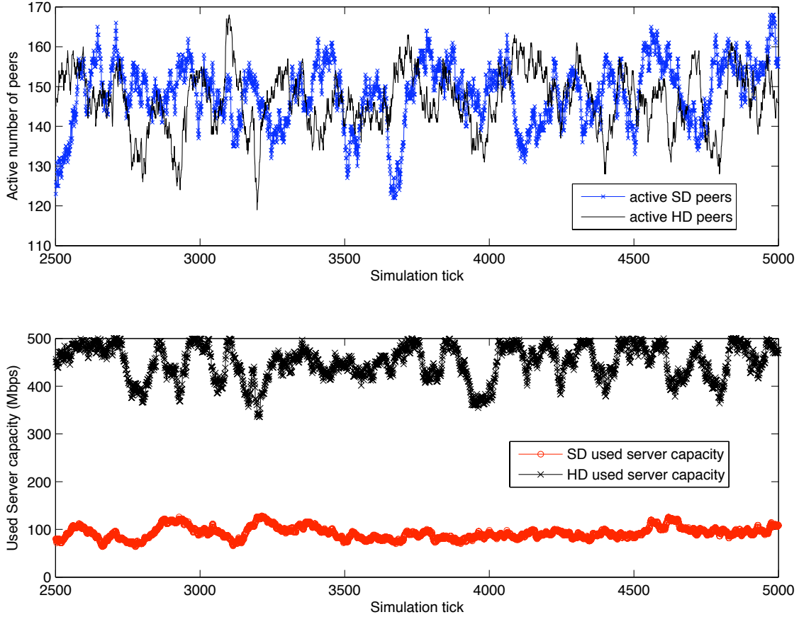
Fig. 12 Comparison of server utilization of SD and HD as a function of time: Z_r = \frac{5}{6} , Z_c = 1 , R_p = 0.01
