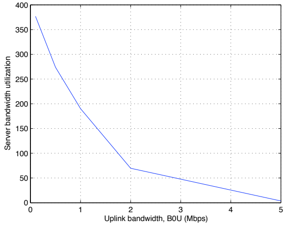
Fig. 10 Server bandwidth utilization (Mbps) vs increasing uplink b/w
