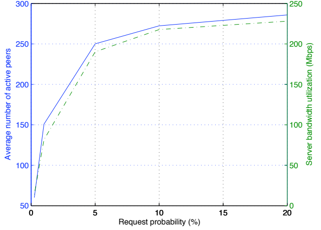
Fig. 9 Average number of active peers (left y-axis) and Server bandwidth utilization (right y-axis -) vs Request probability
