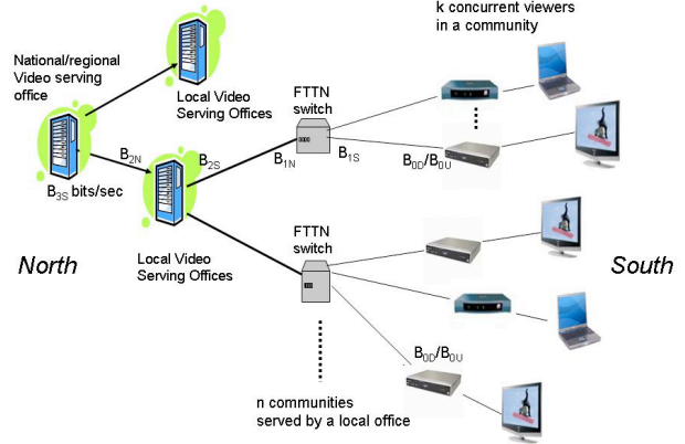
Fig. 2 Physical Model for IPTV Service
