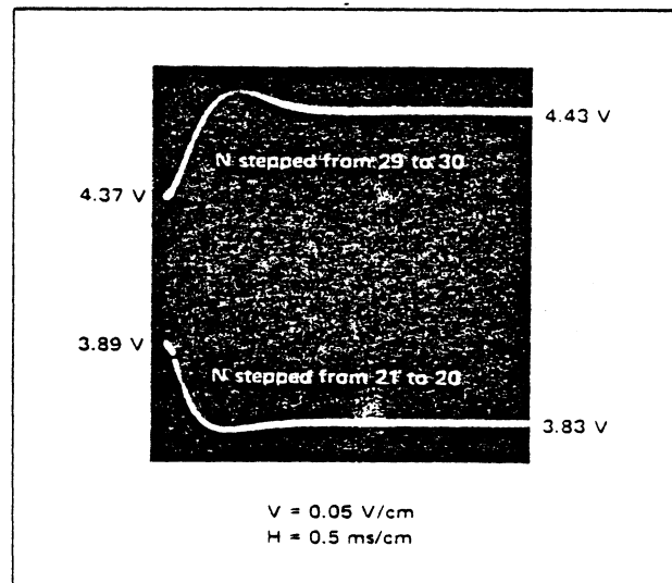
FIGURE 14 – VCM Control Voltage (Frequency) Transient
