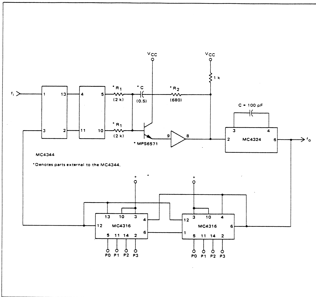
FIGURE 10 – Circuit Diagram of Type 2 Phase Locked Loop
