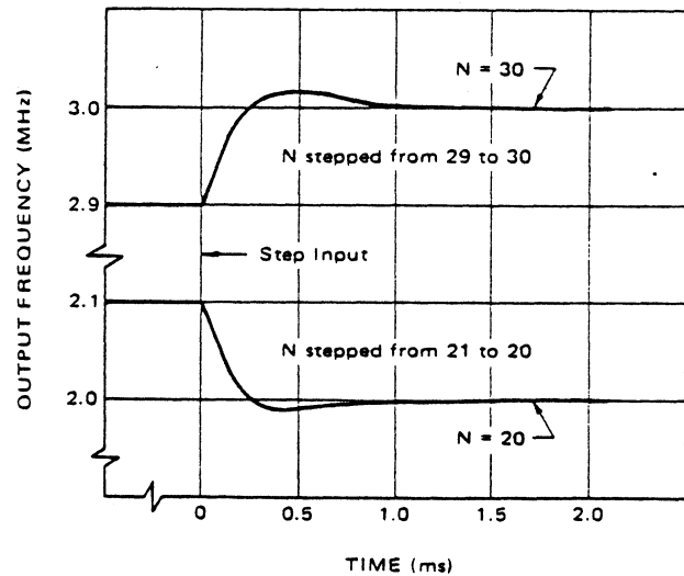
FIGURE 13 – Frequency-Time Response
