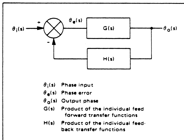
FIGURE 1 - Feedback System
