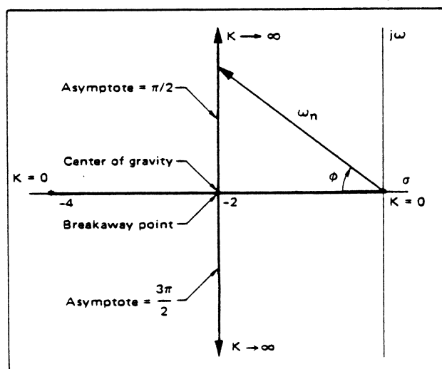
FIGURE 3 - Type 1 Second Order Root Locus Contour
