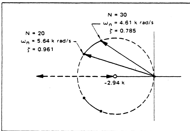
FIGURE 12 – Root Locus Variation
