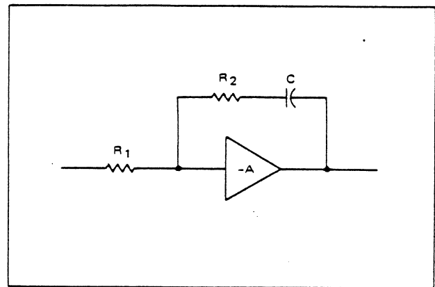
FIGURE 9 - Active Filter Design
